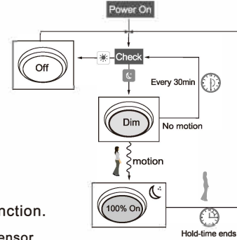
1 goes in cycle at night ... 100% on when movement detected, and dims to 10% in long absence. When the natural light level exceeds setpoint off to light, the light will turn off even if when the space is occupied. The light automatically turns on at 10% when natural light is insufficient (no motion).
